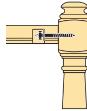
C-3302 Rail Bolt Fastener Includes Fastener, Washer, Nut and Plugs
