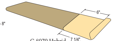
C-8070 Hybrid Reversible (Oak Reveal) Tread 1-1/32" x 11-1/2"
