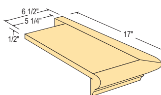
C-8071 Tread Cap with Mitered Return Nosing and Cove Left or Right (RH shown)
