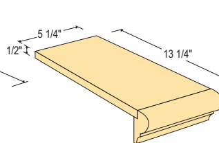
C-8072 Tread Cap with Nosing and Cove
