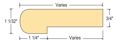
C-8090 - 3-1/2" Wide C-8590 - 5-1/4" Wide C-8690 - 6-1/2" Wide Landing Tread
