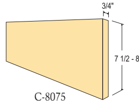
C-8075 Riser 3/4" x 7-1/2" and 8"
