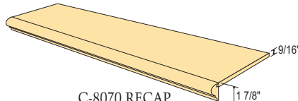
C-8070 RECAP Reversible Remodeling Tread with Nosing and Cove 9/16" x 11-1/2"
