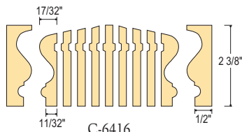
C-6416 Bending Rail with Bending Mould
