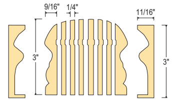
C-6716 Bending Rail with Bending Mould
