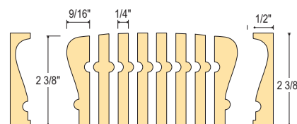
C-6216 Bending Rail with Bending Mould
