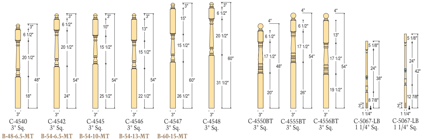
Newels at right are available in 2 options. For Ball Top specify (BT)
