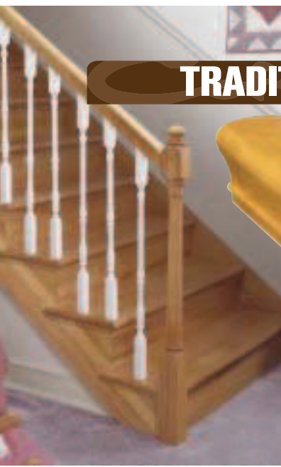
Shown: C-6010 P Handrail, C-5067 Balusters, C-4040 Starting Newel.
